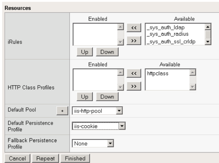
Figure 2.6 Adding the Pool and Persistence profile to the virtual server
