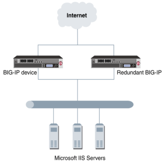
Figure 1 Example Configuration with a redundant BIG-IP system and Microsoft IIS servers
