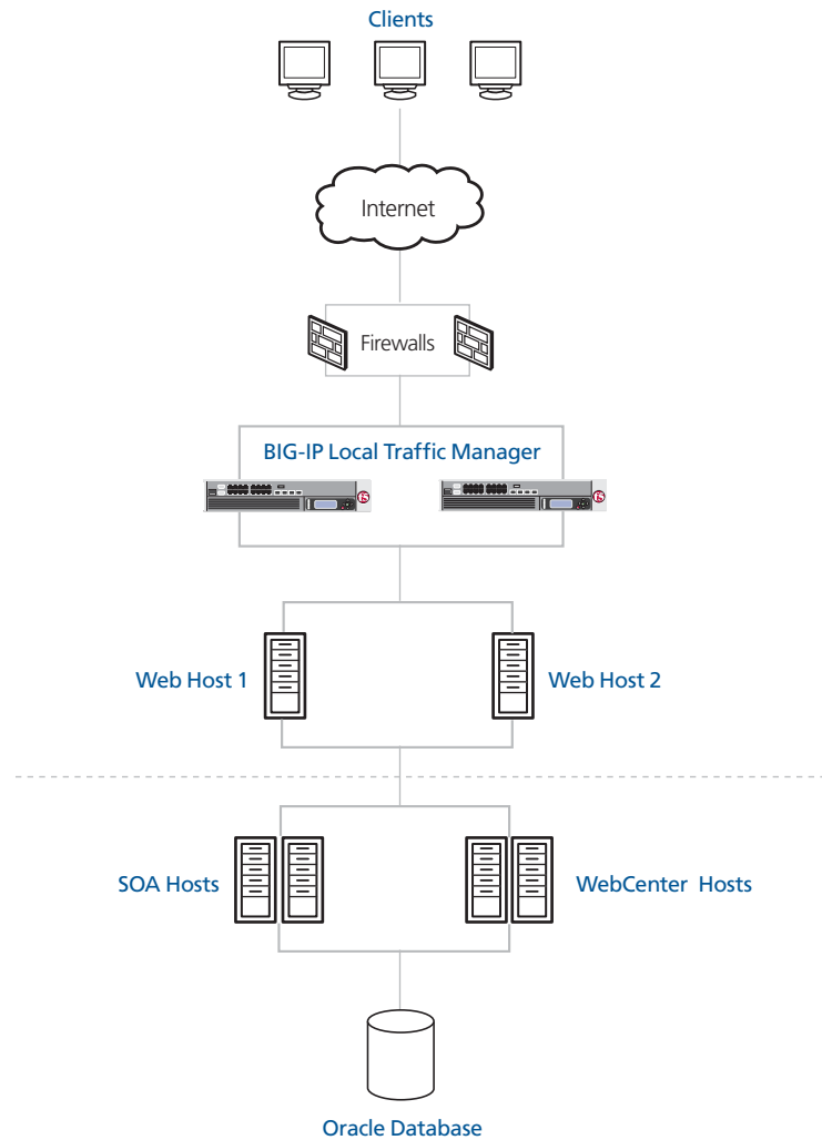
Figure 1 F5 - Oracle WebCenter logical configuration example
