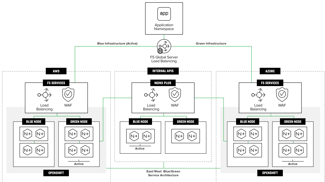
Figure 1: Blue/green deployments extend past the user interface as applications grow and integrate with other applications. Leverage API calls to speed up traffic redirection or failing back if you run into issues.
