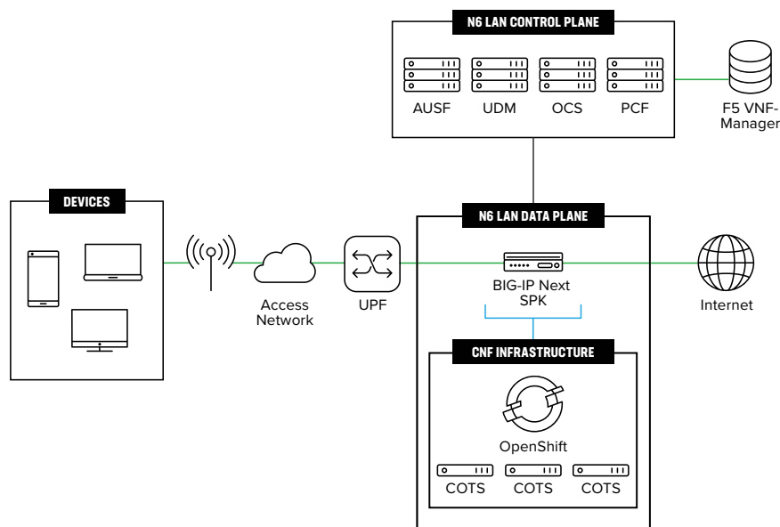
Figure 2: F5's consolidated N6 LAN solution
