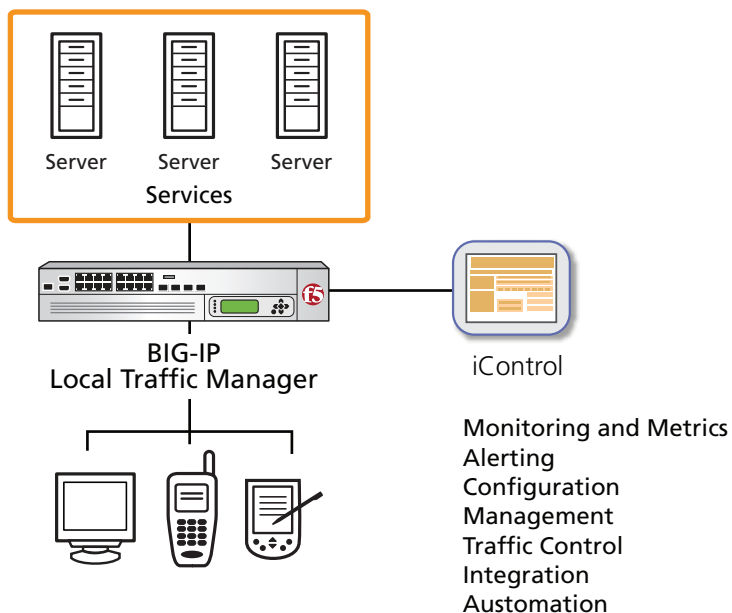
Figure 1: iControl services
