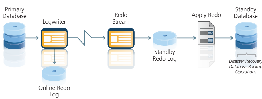
Figure 2: Typical Data Guard configuration
